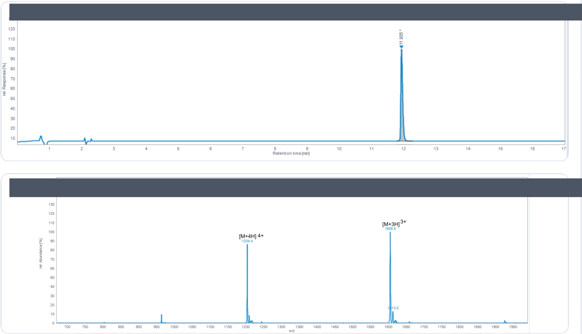
HPLC Chromatogram · Retention Time 11.925 min
