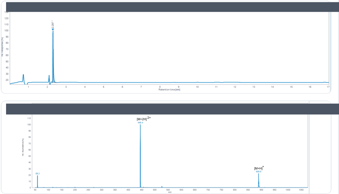
HPLC Chromatogram · Retention Time 2.297 min
