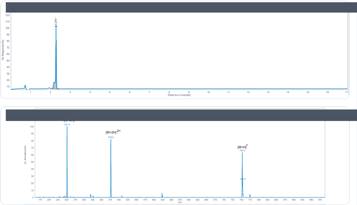
HPLC Chromatogram · Retention Time 2.278 min
