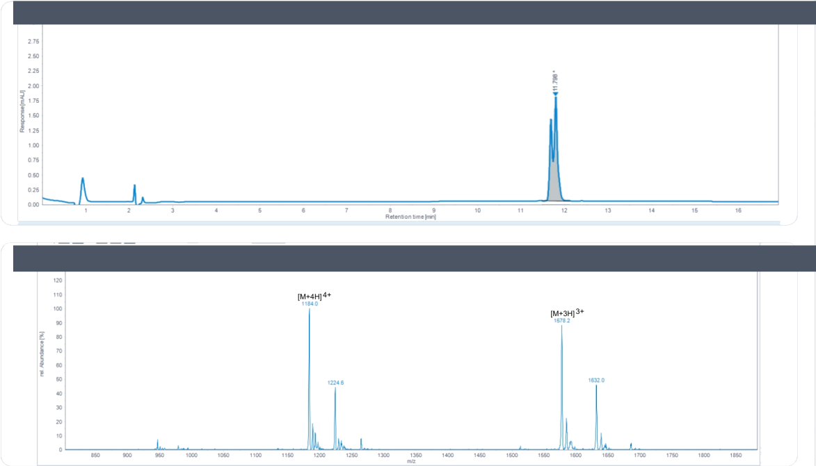
HPLC Chromatogram · Retention Time 11.798 min
