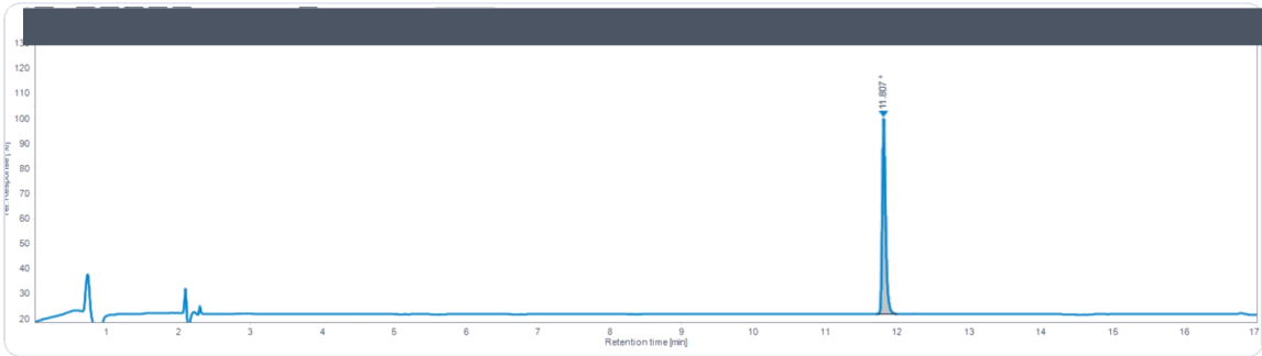
HPLC Chromatogram · Retention Time 11.807 min
