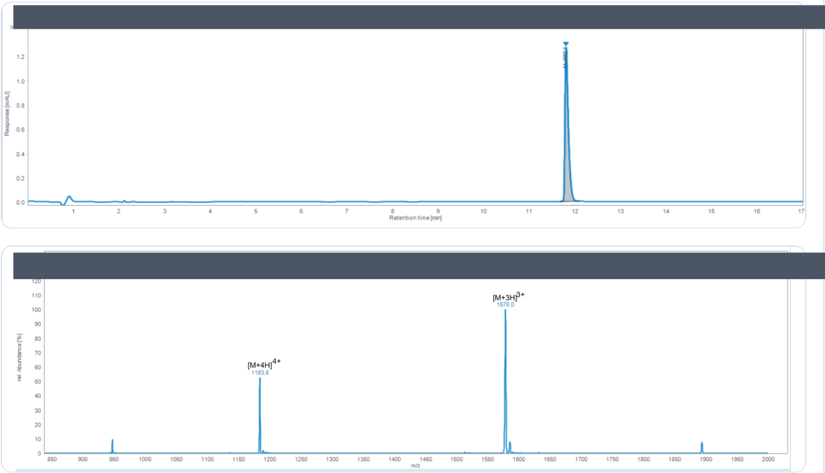
HPLC Chromatogram · Retention Time 11.802 min
