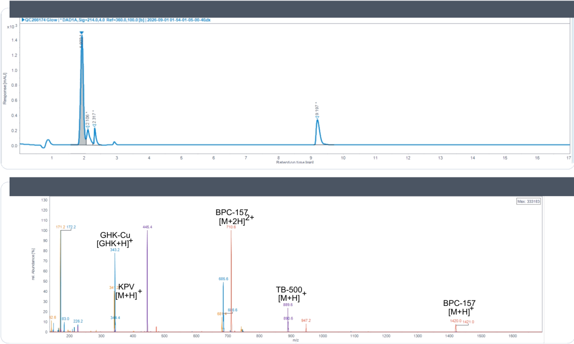
HPLC Chromatogram · Retention Time 1.922, 2.106, 2.317, 9.197 min
