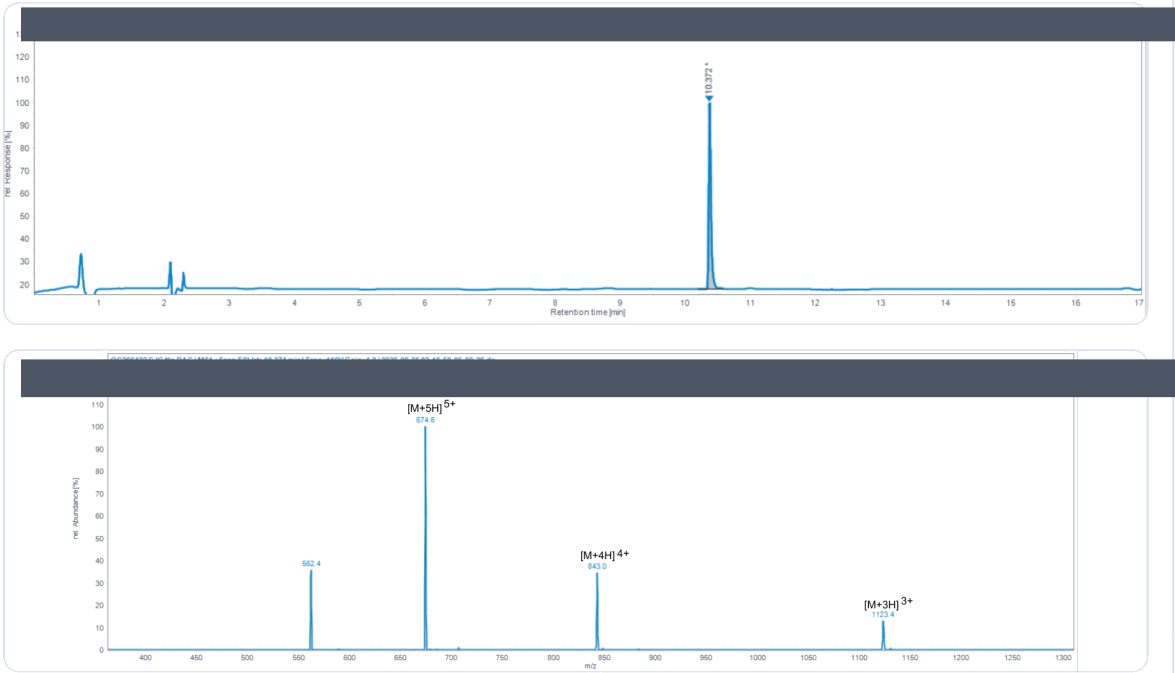
HPLC Chromatogram · Retention Time 10.372 min
