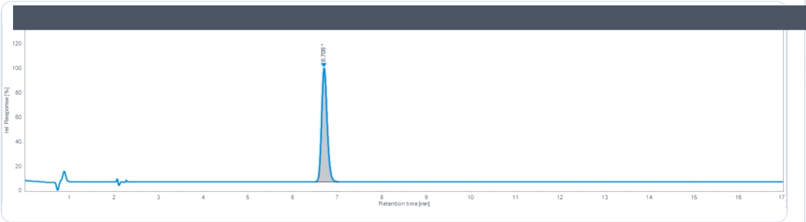
HPLC Chromatogram · Retention Time 6.708 min
