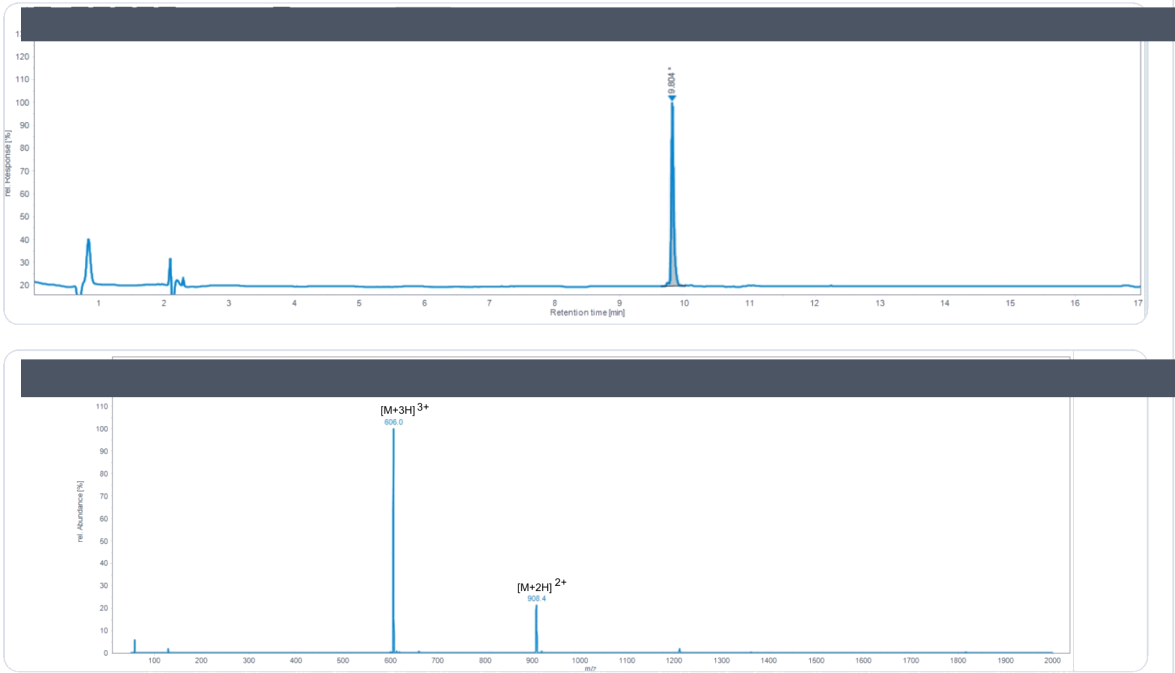
HPLC Chromatogram · Retention Time 9.804 min
