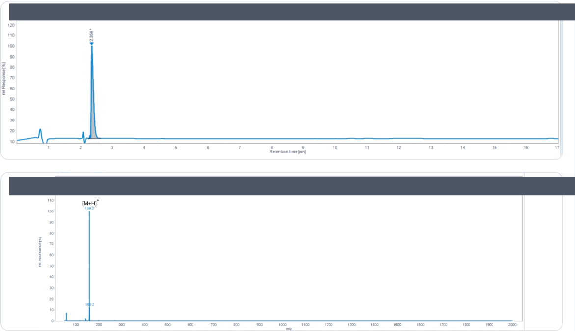
HPLC Chromatogram · Retention Time 2.354 min
